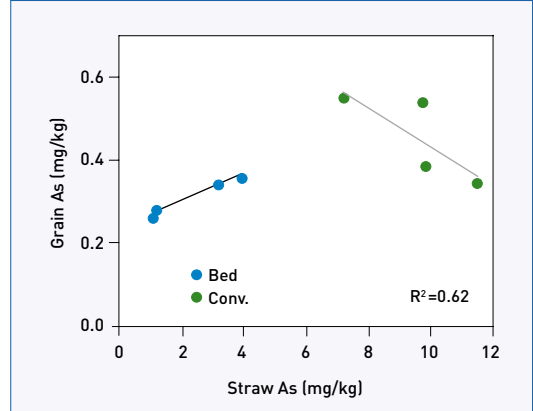
Figure 12. Relationship between arsenic in rice grain and straw for bed and conventional production methods
