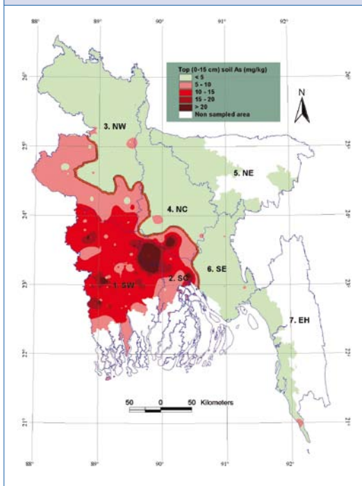
Figure 1. Kriged map of surface soil (0-15 cm) As content; the heavy red line delineates the 5 mg kg -1 boundary
