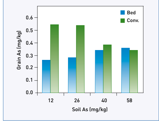
Figure 11A. Effect of soil As content on arsenic levels in rice grain
