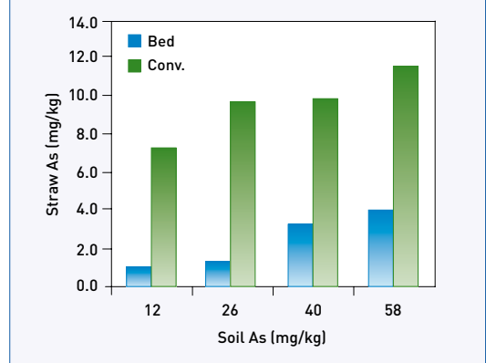
Figure 11B. Effect of soil As content on arsenic levels in rice straw
